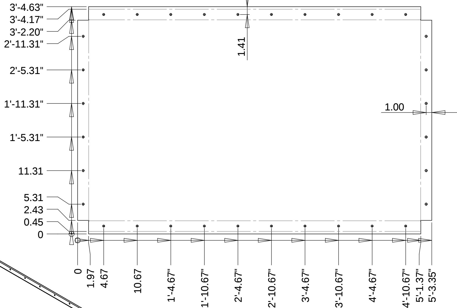
Flat Pattern
